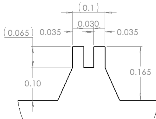
DETAIL B SCALE 7 : 1
